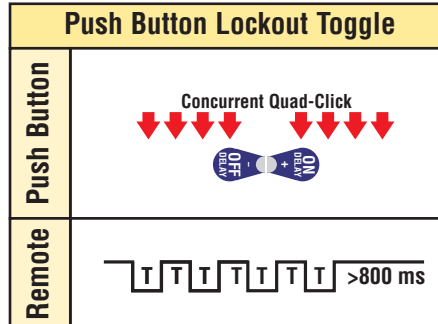
Figure 16. Lockout toggle
